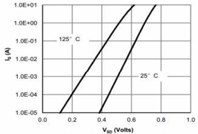
Figure 6: Body-Diode Characteristics
