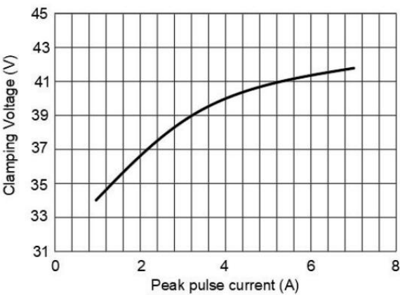
FIG4: Clamping Voltage vs. Peak Pulse Current
