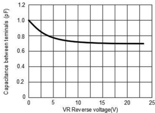
FIG3: Capacitance between teminals charateristics
