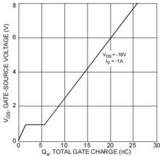
Fig. 14 Gate-Charge Characteristics
